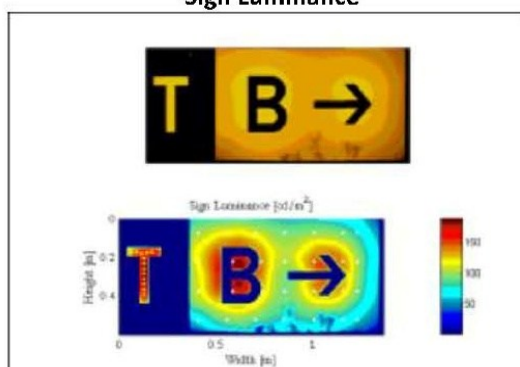
Sign Luminance
