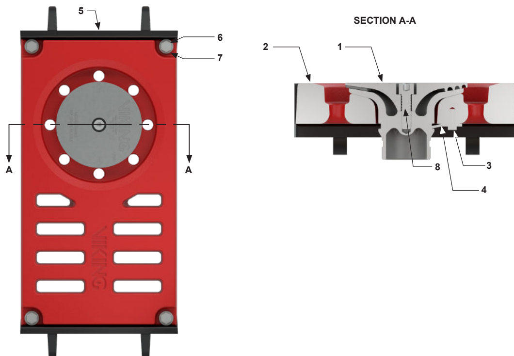
Figure 13.1.1: Replacement Parts
